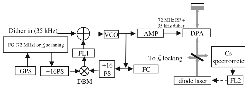
FIGURE 4 Frequency tuning, modulation and stabilization of double-pass AOM (DPA) system. FG – function generator which the output frequency could either be fixed at 72 MHz or be linearly scanned; f_n – absolute frequency of the n th comb mode; VCO – voltage controlled oscillator; AMP – amplifier; FC – frequency counter; PS – prescaler; DBM – double balance mixer; FL – feedback loop
