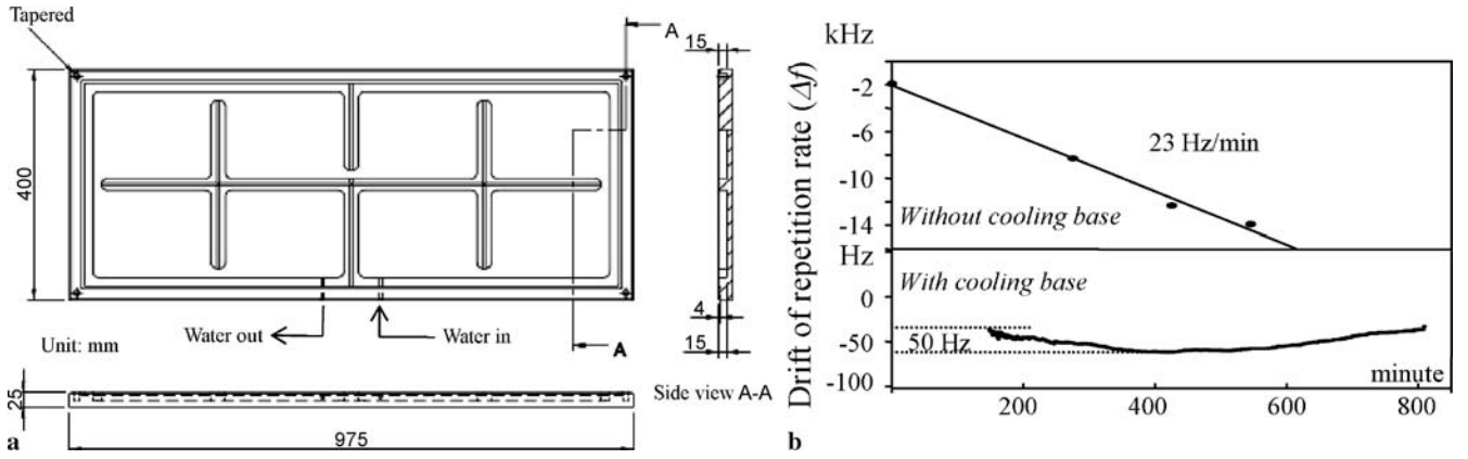
FIGURE 3 (a) Particular-designed cooling base which was installed beneath the comb laser. (b) The repetition-rate drifted 18 kHz during a 13 h period (upper panel), and was reduced two orders of magnitude after installing the cooling base (lower panel)
